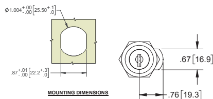
MOUNTING DIMENSIONS
