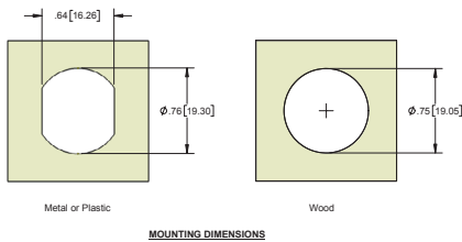
MOUNTING DIMENSIONS
