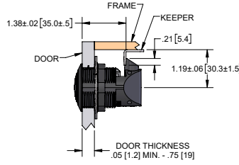
SIDE VIEW CUT-OUT DETAILS
