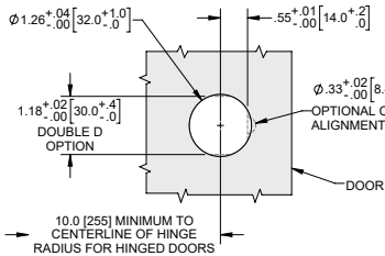
FRONT VIEW DOOR CUT-OUT DETAILS
