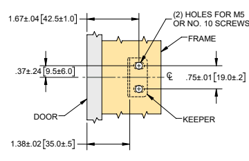
TOP VIEW KEEPER MOUNTING DETAILS
