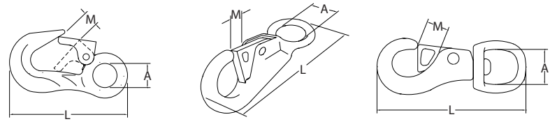
part no. 2311
