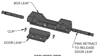
EXPLODED VIEW
