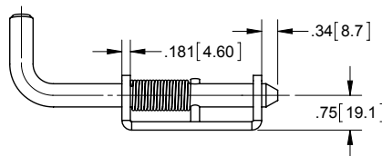
RETRACTED BOLT
