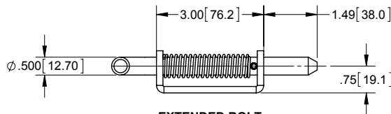
EXTENDED BOLT
