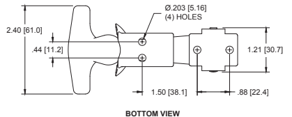
LATCH WITH LONG KEEPER
