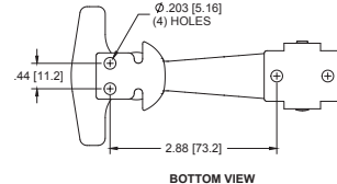
LATCH WITH SHORT KEEPER
