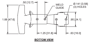
LATCH WITH LONG KEEPER
