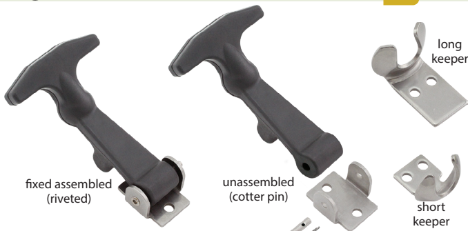
LATCH WITH LONG KEEPER
