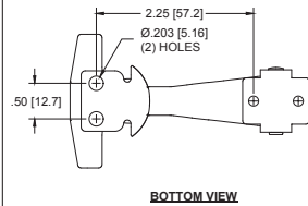
LATCH WITH SHORT KEEPER
