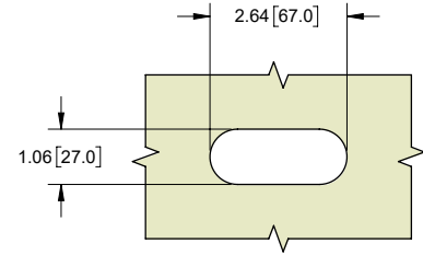
MOUNTING DIMENSIONS
