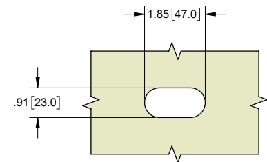
MOUNTING DIMENSIONS
