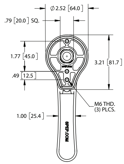
MOUNTING DIMENSIONS
