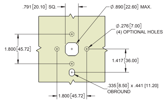
MOUNTING DIMENSIONS
