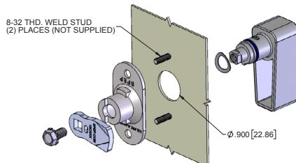
MOUNTING DIMENSIONS
