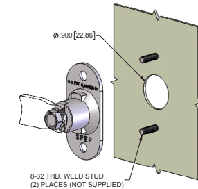
MOUNTING DIMENSIONS
